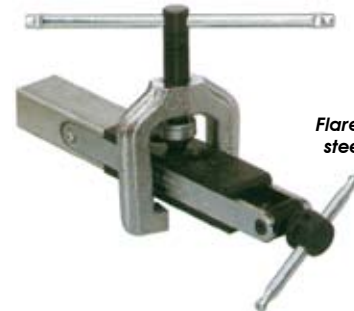
Flares rolled out above die by smooth faceted cone. Makes stronger flares.
